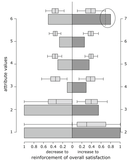
Fig. 10 OrdEval results for Project management
